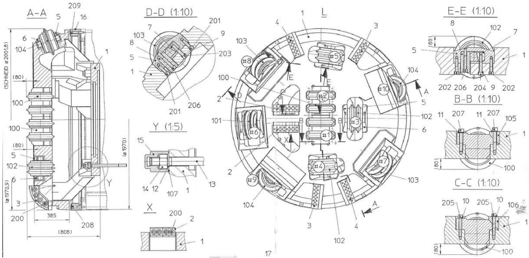
AVN1500 TB FRONT, CUTTERHEAD
